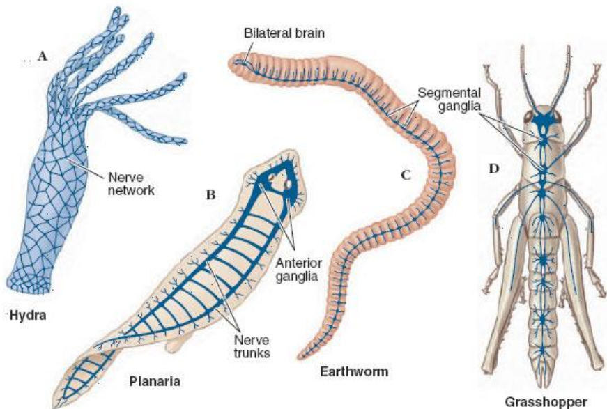
Gambar 3.3. Sistem saraf Invertebrata
