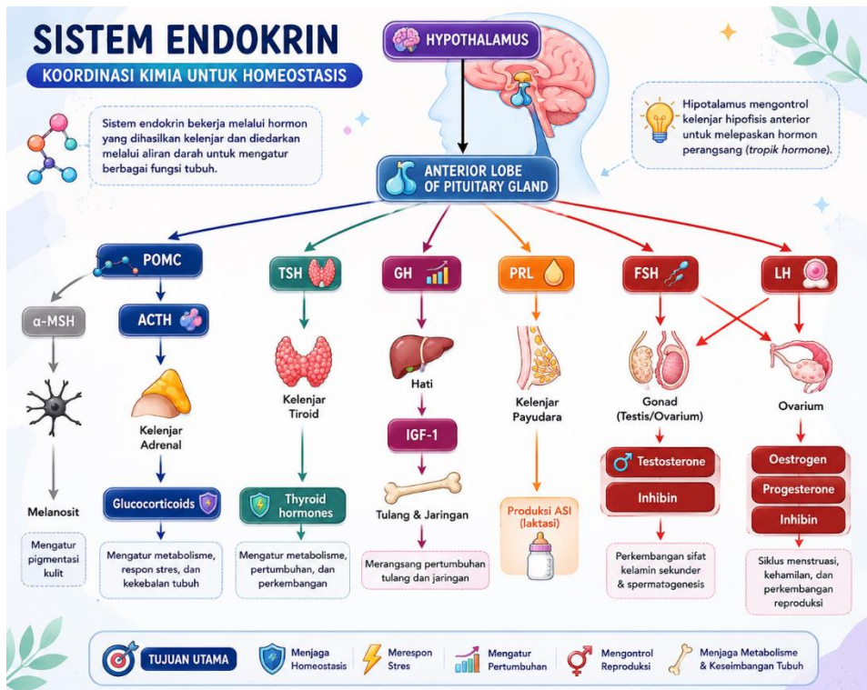
Gambar 6.1 Diagram hypothalamus pituitary axis
